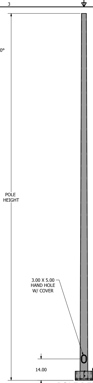
POLE DETAIL
