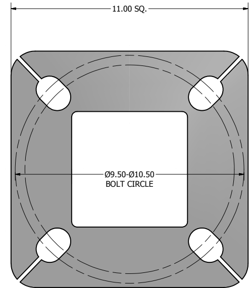
11.00 X 11.00 X 1.00 BASE PLATE
