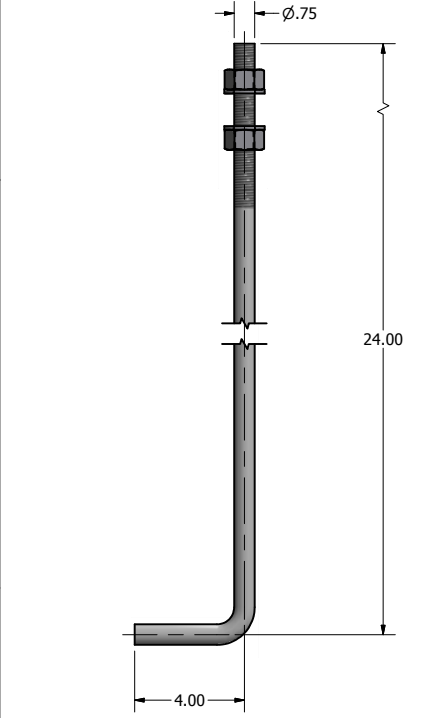
Ø.75 X 28.00 ANCHOR BOLT
