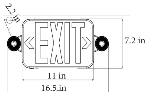
Wall mount
