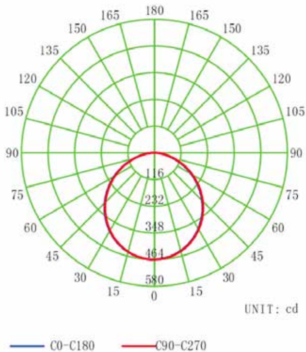
LUMINOUS INTENSITY DISTRIBUTION DIAGRAM
