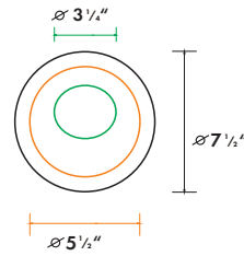
6"Round WallWasher
