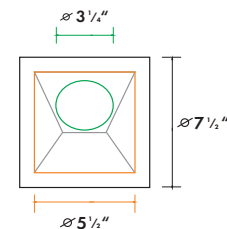
6"Square WallWasher
