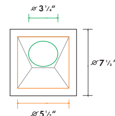
6"Square WallWasher
