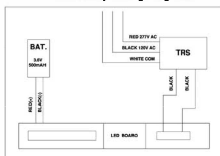
Exit Battery Wiring Diagram:
