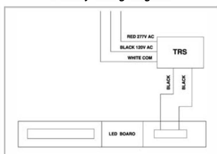
AC Only Wiring Diagram:
